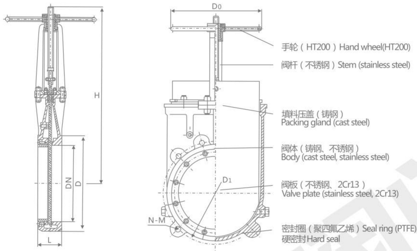
主要性能规范 Main Performance Specifications
